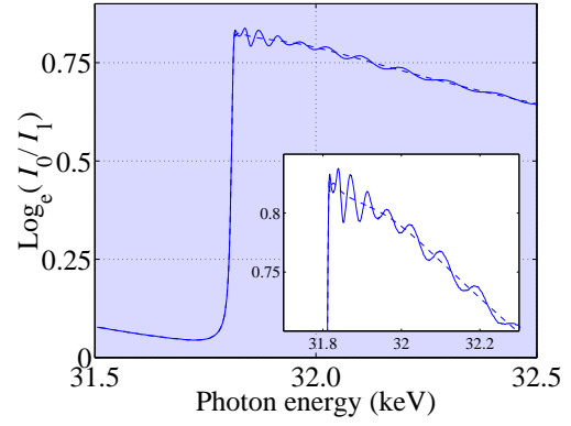
CdTe, Nano-crystalline
