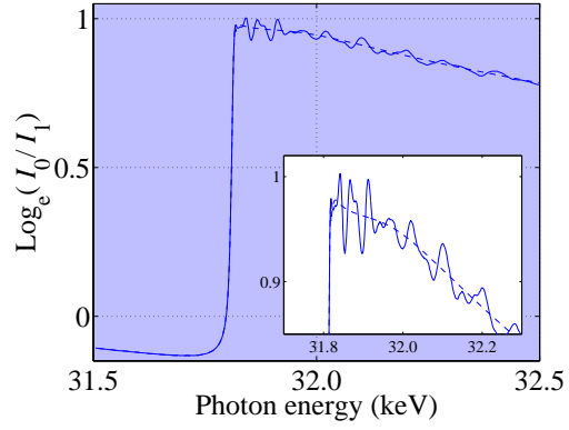
CdTe, bulk
