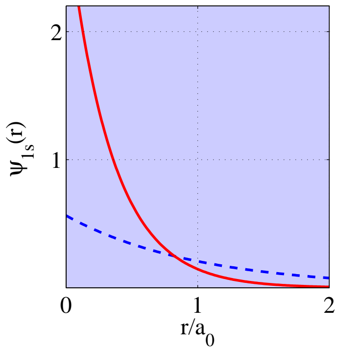
1s Wavefunction
