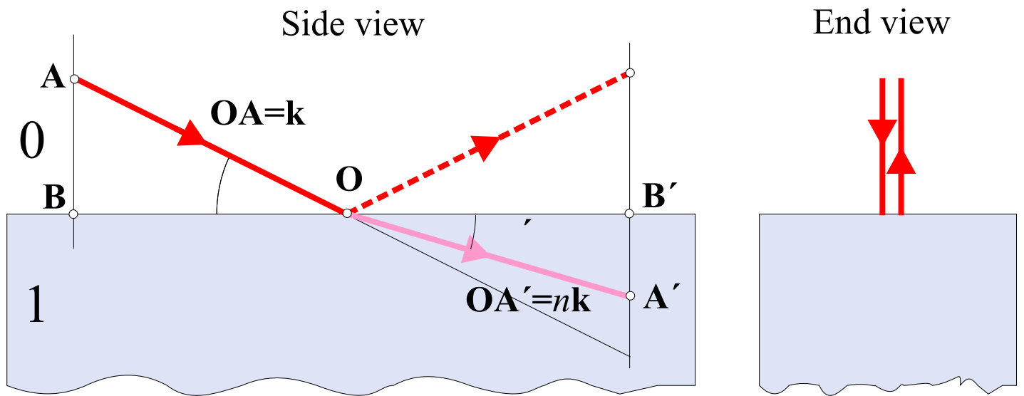
(a) Infinitely thick slab
